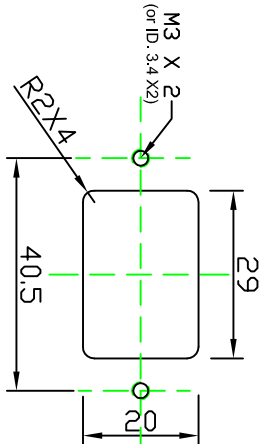
Panel Cut-out Size for FI-10 (for Front mounting Use)
